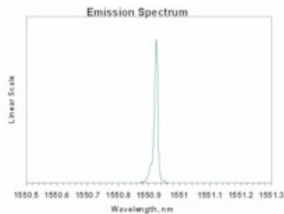
DFB Laser Spectrum
