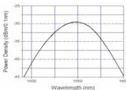
SLD Light Source Spectrum
