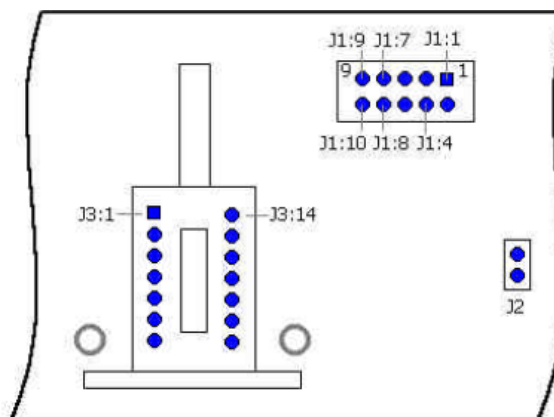
Top view of connectors layout
