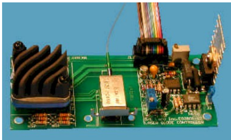
Figure1. Laser Diode Controller for DIP Type Laser Diode
