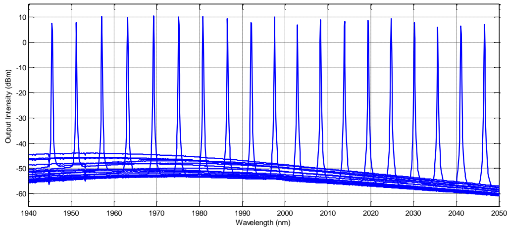
Output spectrum of OEBS-TLS-STD at 2000 nm
