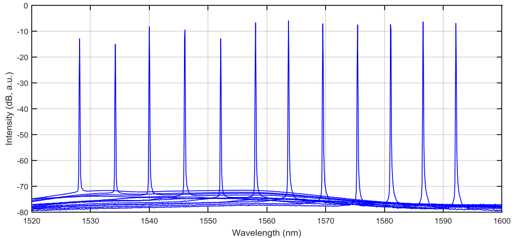
Output spectrum of OEBS-TLS-STD at 1550 nm
