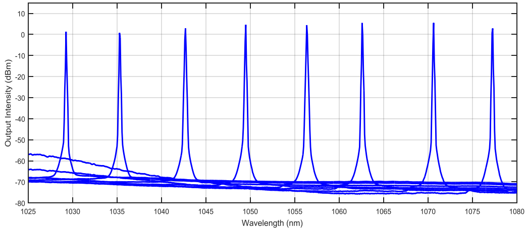
Output spectrum of OEBS-TLS-STD at 1060 nm
