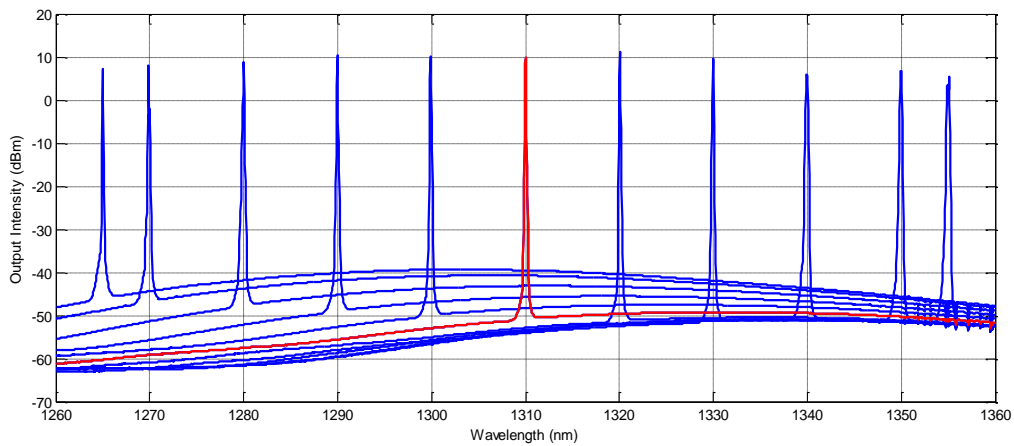
Output spectrum of OEBS-TLS-STD at 1310 nm
