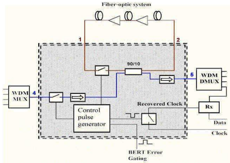
Fig2. System Configuration Diagram
